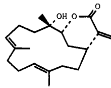
Uchio's toxin
