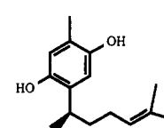
curcuhydroquinone
