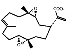
bis-epoxide precursor
