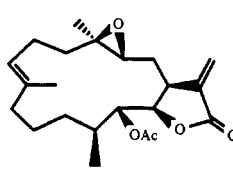
eupalmerin acetate
