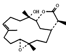
dihydroflexibilide
